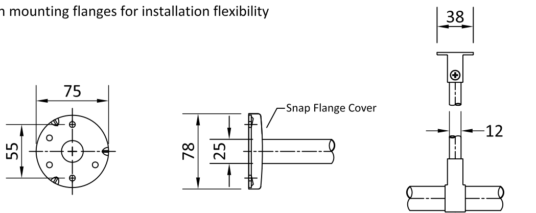
WALL & CEILING FIXING DETAIL (Scale 1:4)
