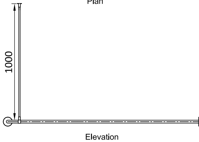
SHOWER CURTAIN RAIL (Scale 1:20)
