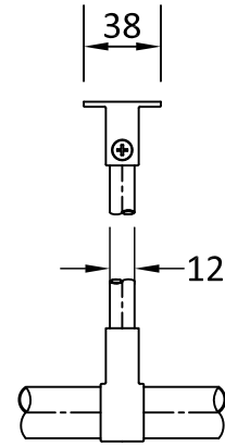
Ceiling Support Bracket
