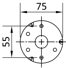
Mounting Flange
