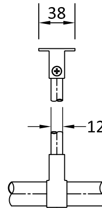
Ceiling Support Bracket
